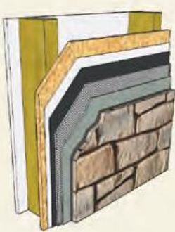
Wood Stud Installation Sheathing Weather resistant barrier Weather resistant barrier Metal lath Scratch coat Setting bed Dutch Quality Stone™
