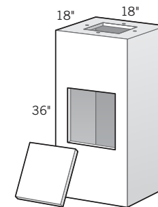
Column with End Cap 18"D × 18"L × 36"H • OLPLS1836 Instantly build perfect stone or brick columns. Column ships with access panel. Designed with top and bottom flange for attaching masonry anchor or bolting.
