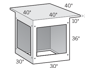
90° Corner Cabinet with 10" Cantilever on Two Sides 30"D × 30"L × 36"H • OLPLSCHBC
